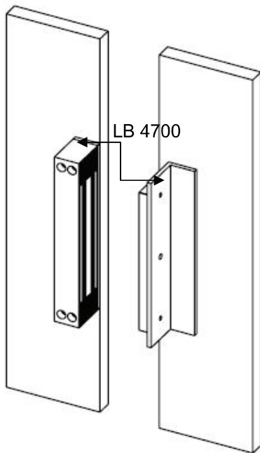
EM4700S LSS/ Side Mount
