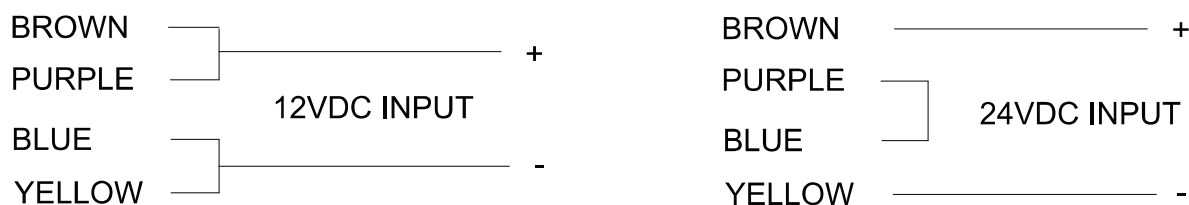
Illustration of wiring for EM4700FS
